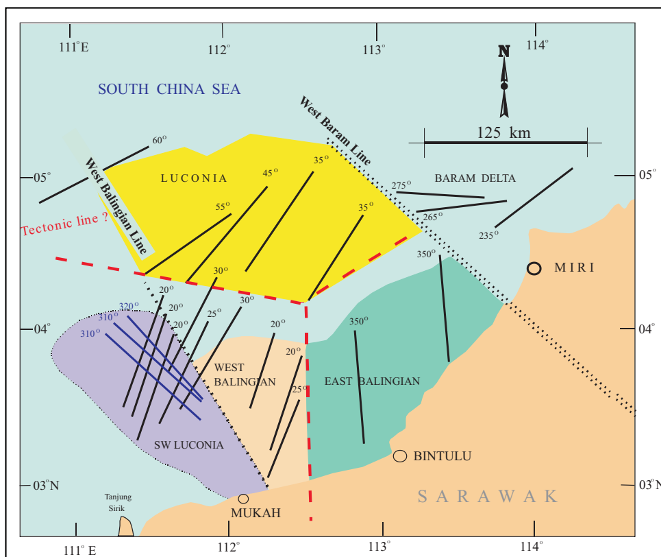
Figure 4. The Sarawak Basin stress pattern constructed from wellbore breakout study. A good correlation exist between S_{Hmax} orientation pattern and the established tectono-stratigraphic provinces. Southwest Luconia possess relics of older S_{Hmax} (blue lines) and younger (black lines) S_{Hmax} orientations occurring in the same wells. Azimuths of the younger S_{Hmax} are similar to that in the neighbouring West Balingian subprovince. Data from Tjia & Idrus Ismail (1994).
