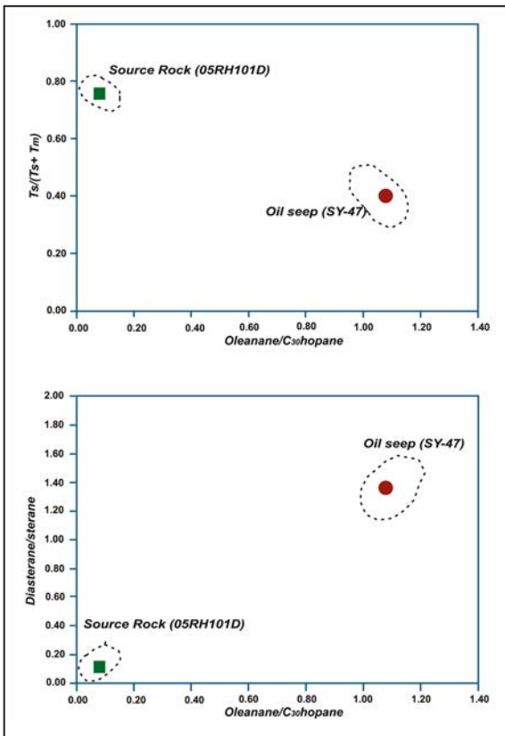
Figure 9. Source rock-oil seep correlation using parameters of: (a) oleanane/C 30 hopane versus Ts/(Ts+Tm) ratios, and (b) oleanane/C 30 hopane versus diasterane/sterane ratios; the result indicates that the oil seep does not appear to perfectly matching with the source rock sample.
