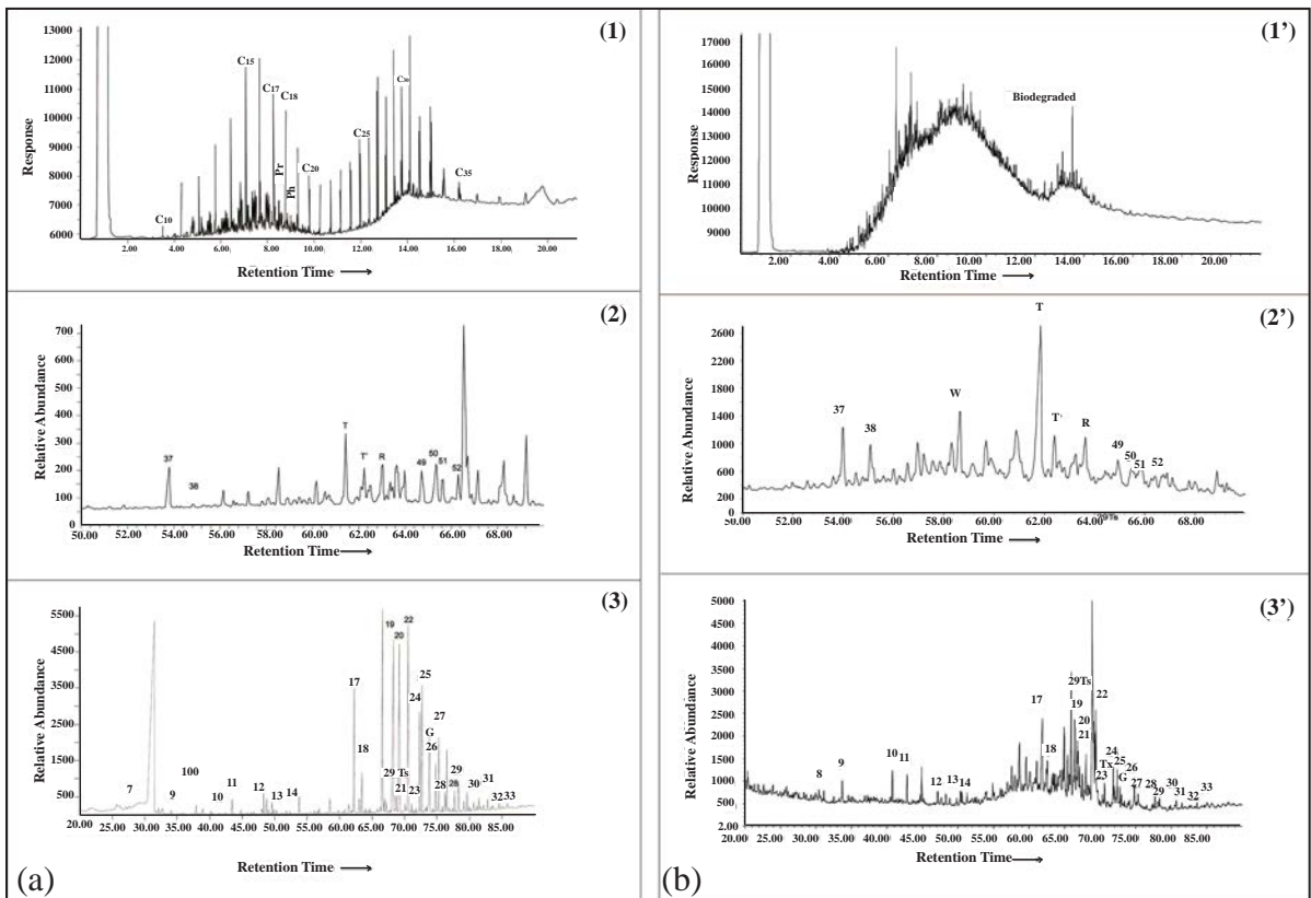
Figure 8. a) Gas chromatography analysis of a rock sample from the Lemau Formation (05RH101D), showing (1) Gas Chromatography-Mass Spectrometry analysis; (2) Saturate Biomarkers m/z 217 Steranes; (3) m/z 191 Triterpanes; b) Oil seep sample (SY-47), showing (1') Gas Chromatography-Mass Spectrometry analysis where the oil appears to have been biodegraded; (2') Saturate Biomarkers m/z 217 Steranes; (3') m/z 191 Triterpanes.
